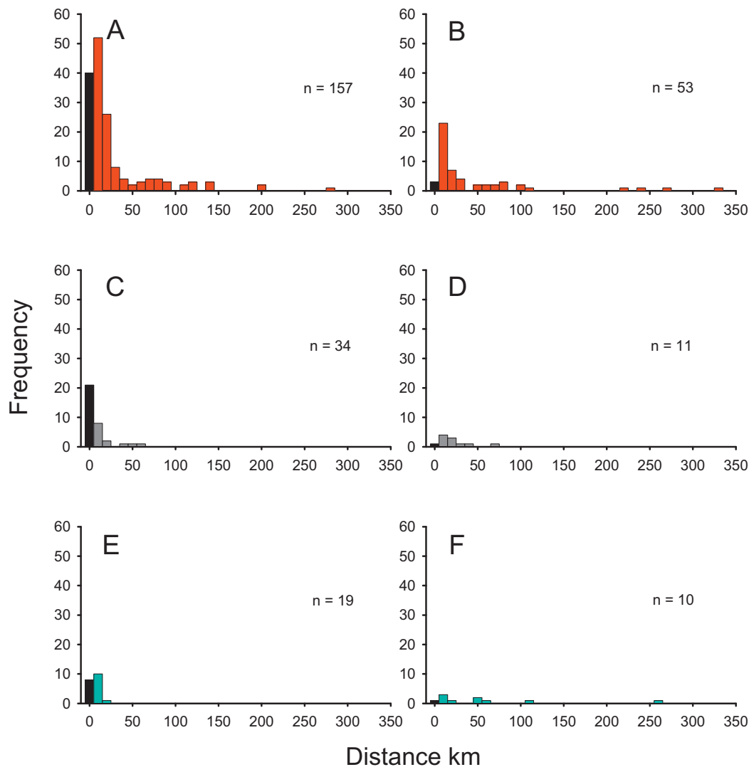
Fig. 5. Frequency distributions of estimated distance moved (km) observed for tagged fish exposed to a hurricane: (A) red snapper, (C) gray triggerfish, and (E) groupers; and frequency distributions of estimated distance moved (km) observed for tagged fish not exposed to a hurricane: (B) red snapper, (D) gray triggerfish, and (F) groupers. Recaptures made at study reefs on tagging trips are shown in black (zero movement).
